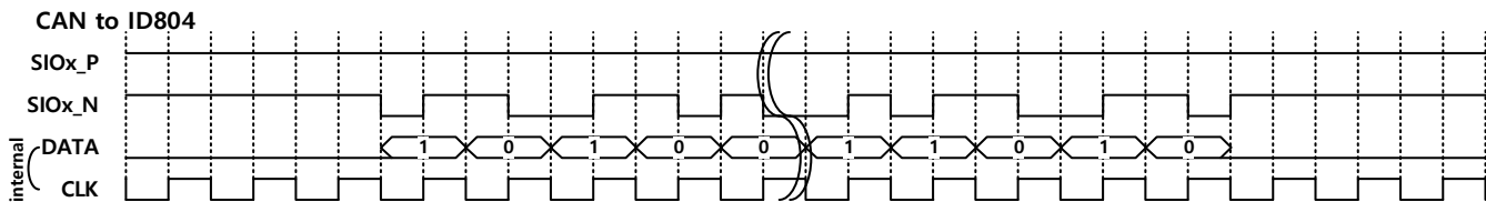
Fig 17. Example of CAN Transceiver to ID804 communication
