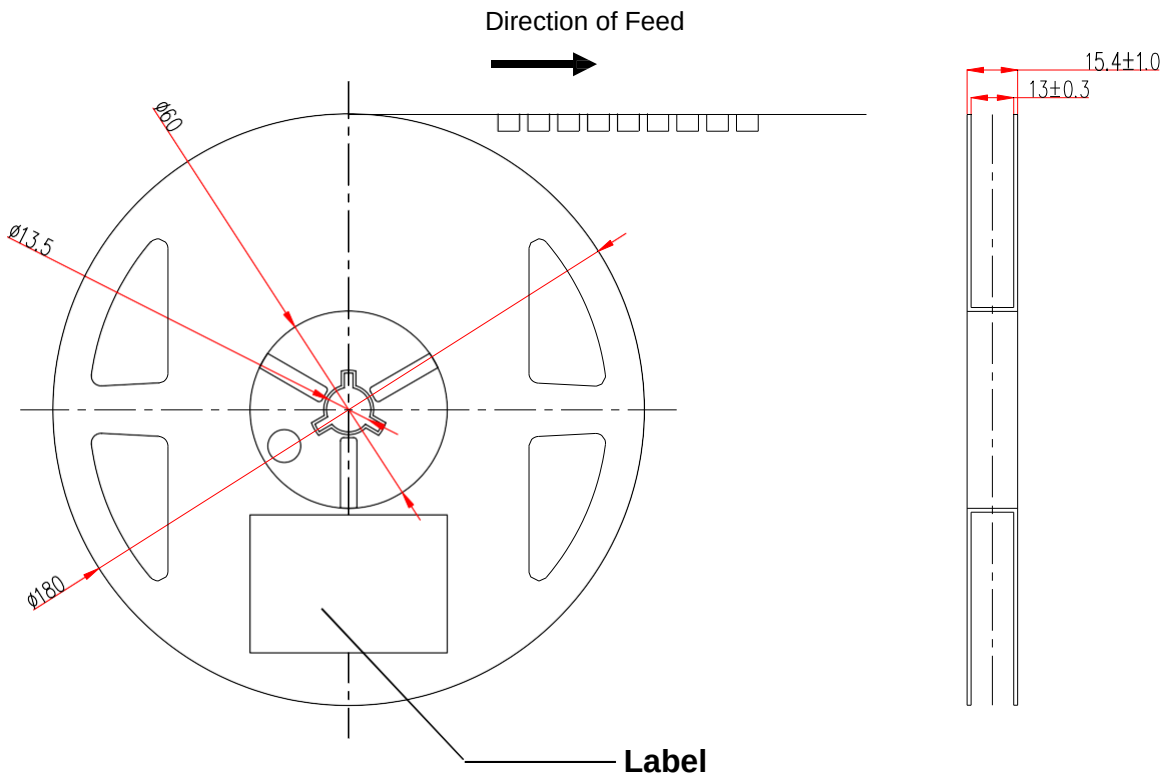
Fig 44. Reel Dimension
