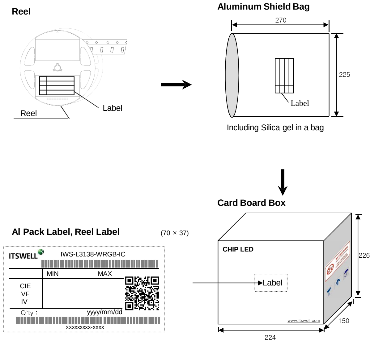
Fig 45. Packing Dimension
