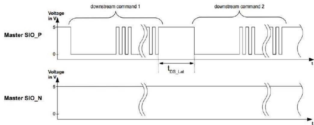
Fig 37. Multiple single ended downstream commands
