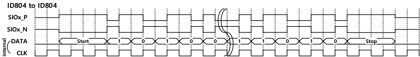
Fig 14. Example of ID804 to ID804 communication
