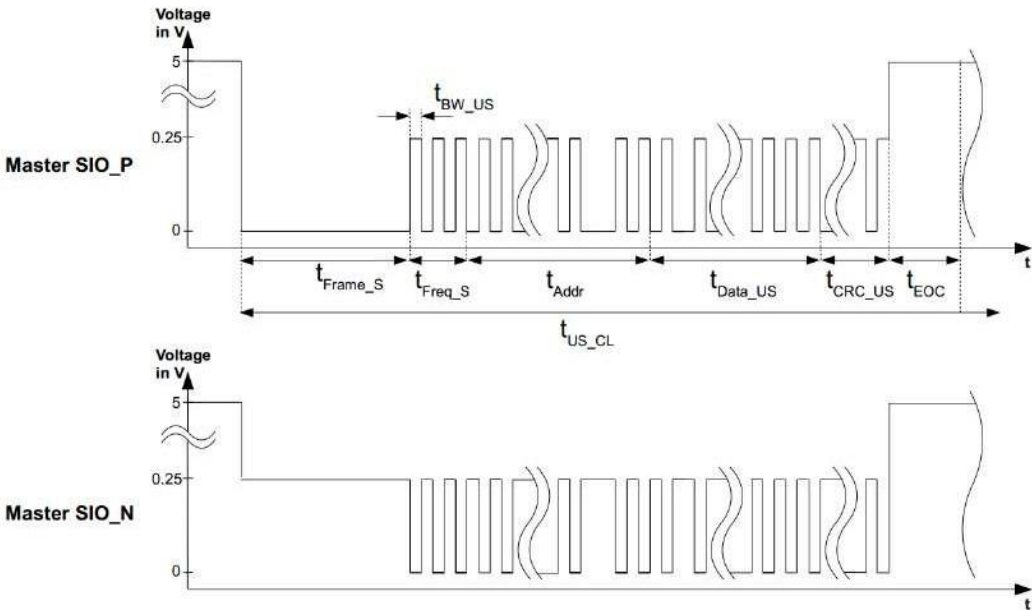
Fig 36. Differential upstream response frame
