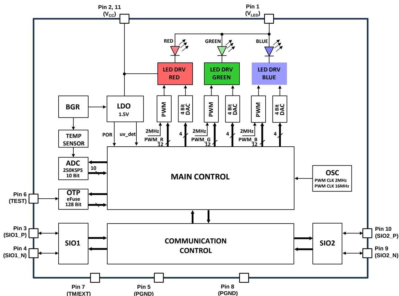
Fig 6. Block Diagram
