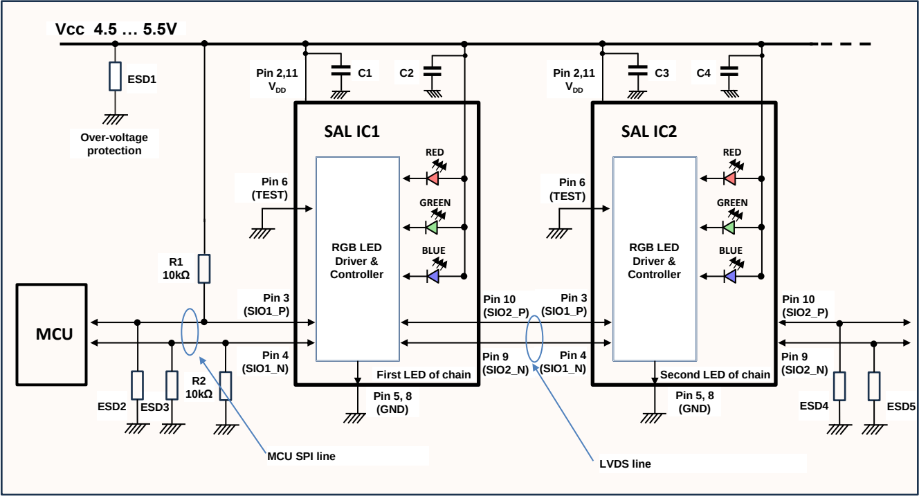
Fig 7. Typical Application Layout
