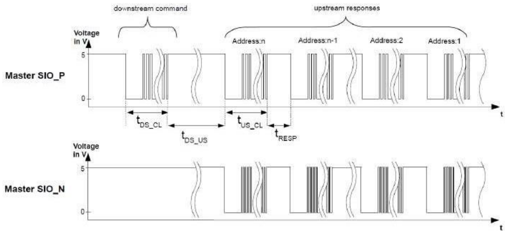
Fig 38. Single ended read command and responses
