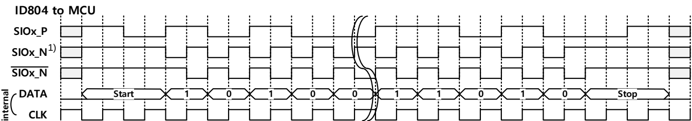
Fig 13. Example of ID804 to MCU communication
