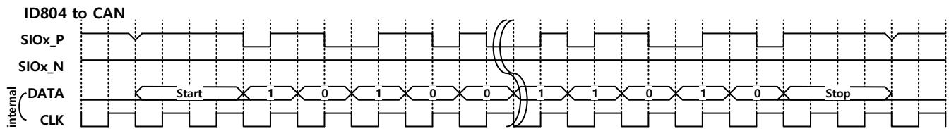
Fig 18. Example of ID804 to CAN Transceiver communication
