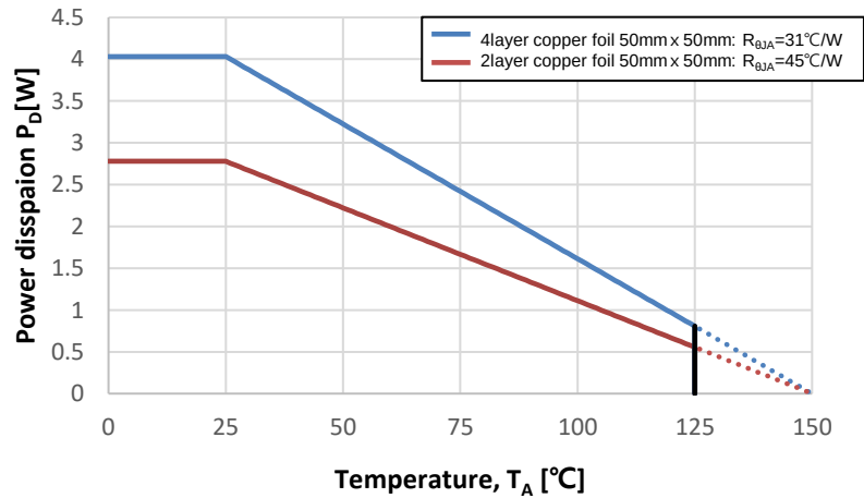
Fig 8. Thermal Considerations
