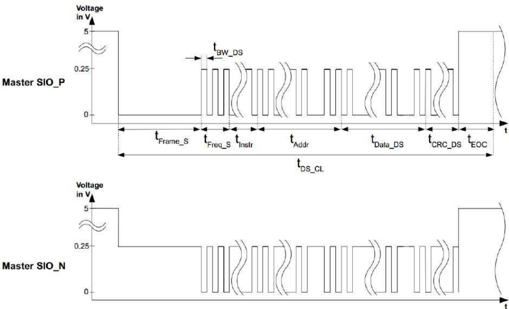
Fig 34. Differential downstream command frame
