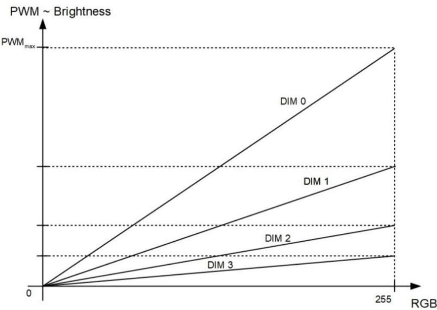
Fig 40. DIM Function for Accurate Low Light Colors
