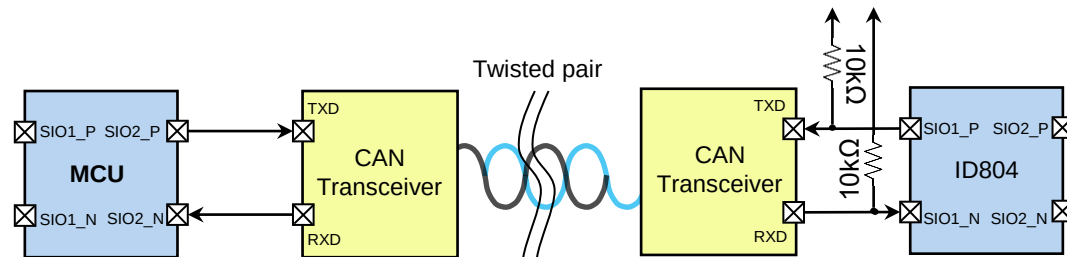
Fig 16. Bi-directional chain example with direct MCU-CAN-FD connection. The MCU needs to implement the Manchester decoder.
