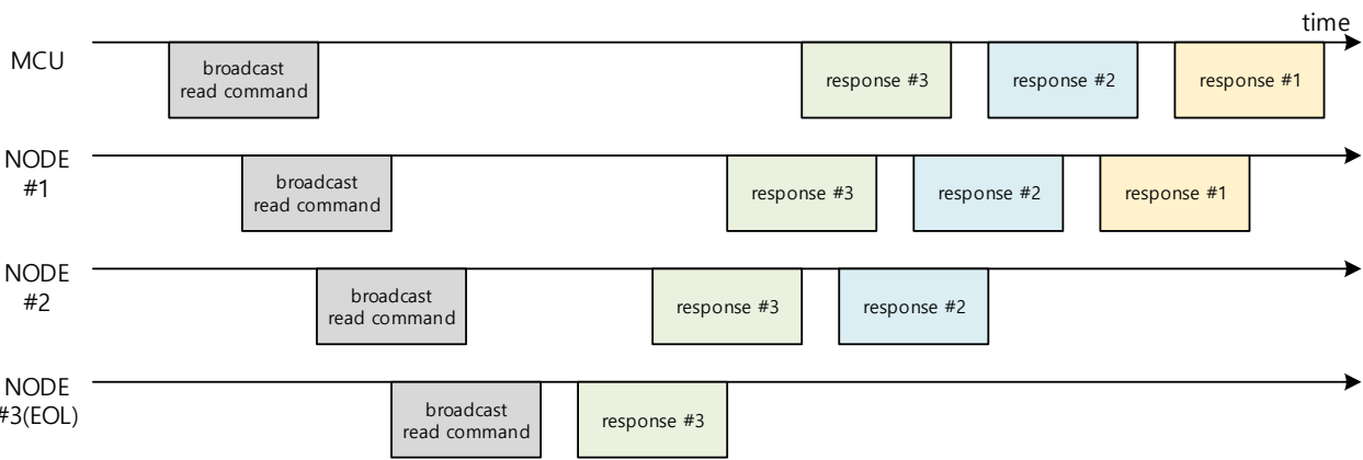
Fig 23. Example of broadcast read(or SR)
